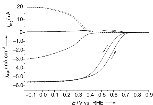
Figure 1. Reduction of \text{O}_2 at a rotating Pt ring/glassy carbon disk electrode supporting [\text{Cu}(\text{Hdatz})]/\text{Vulcan} (solid line) or unmodified Vulcan XC-72 (dashed line) at 1600 rpm in \text{NaClO}_4 (0.1 M) and Britton–Robinson buffer (0.04 M, pH 7.0) saturated with \text{O}_2 . Disk current density ( j_{\text{disk}} ) is shown on the lower half and ring current ( I_{\text{ring}} ) is shown on the upper half of the y-axis. The disk potential was scanned at 5 \text{ mV s}^{-1} ; the ring potential was constant at 1.2 V.
